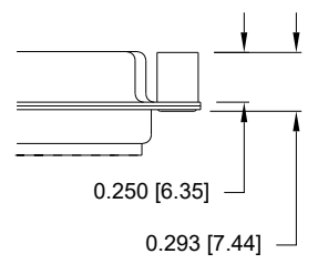
03 ..... 0.250" (MATING SIDE)
