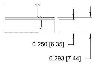
02 ..... 0.250" (SOLDER SIDE)
