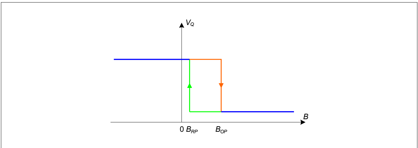
Figure 2-4 Output Signal TLE4964-4M
