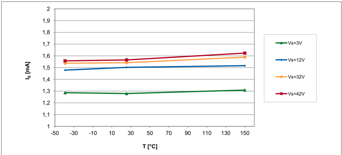
Figure 6-3 Supply Current of the TLE4964-4M over Temperature
