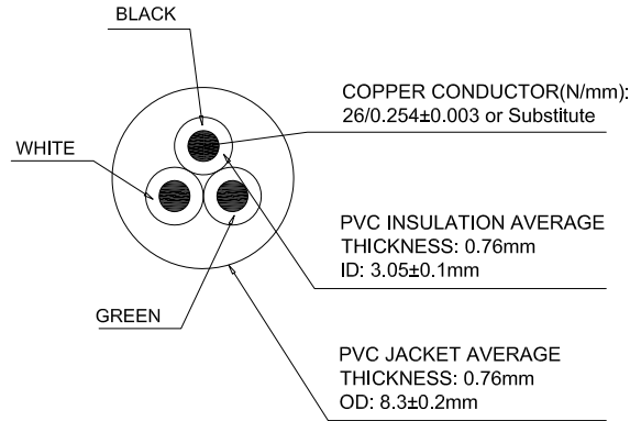
Wire cross section
