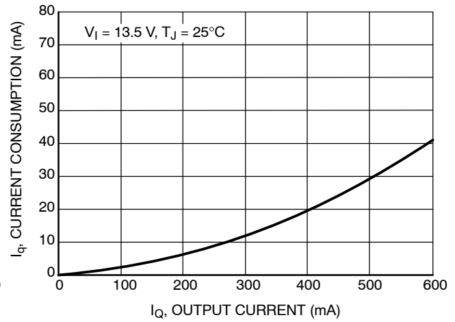
Figure 9. Current Consumption I_{q1} vs. Output Current I_Q
