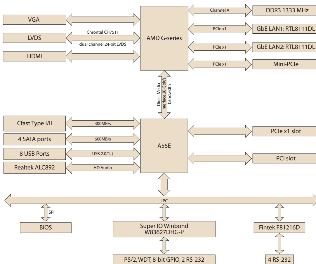
Figure 1.3 AIMB-223 Board Diagram
