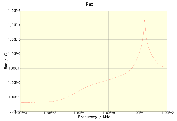
CLF12555T-150M-CA
