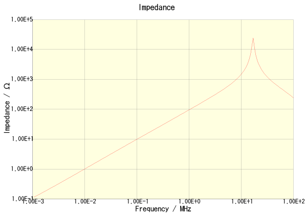
CLF12555T-150M-CA
