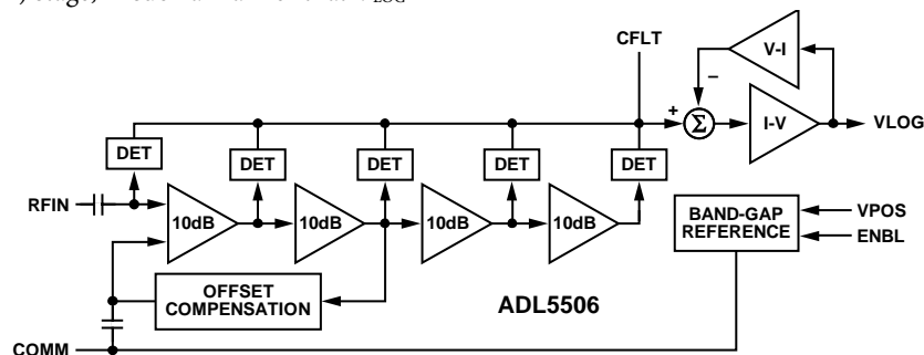
Figure 41. Block Schematic
