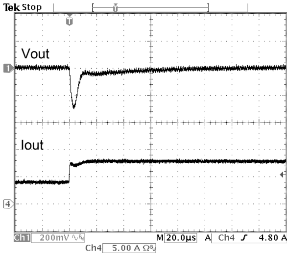
Fig.17: Output voltage response to step load change at 5A/us from 50% to 100% (5.0Vin, 2.75Vout)
