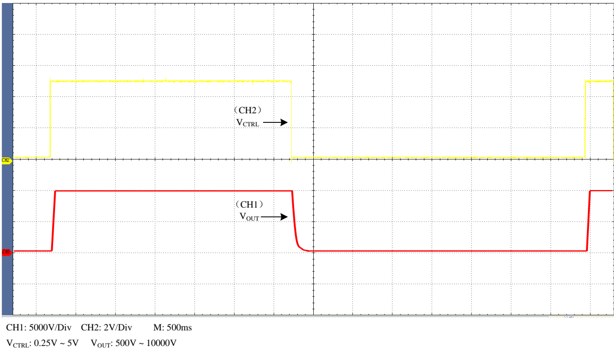
Figure 5. Square Wave
