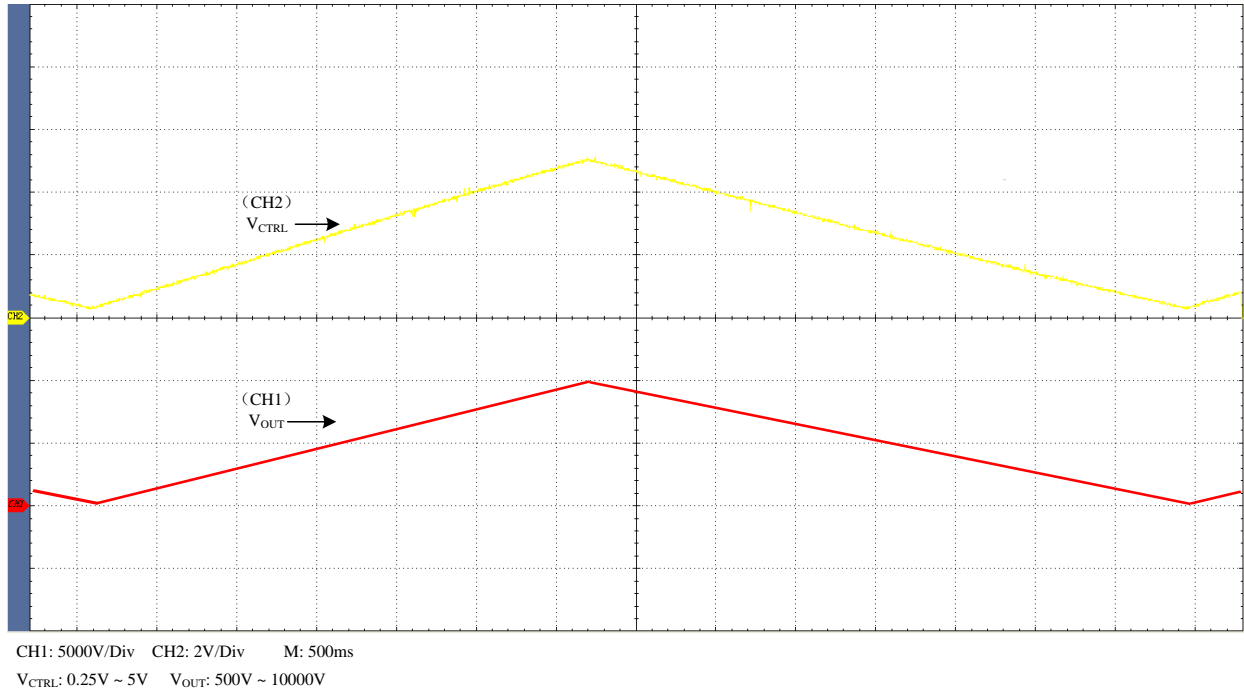
Figure 3. Triangle Wave
