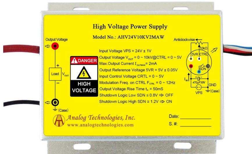
Figure 1. Physical Photo of AHV24V10KV2MAW
