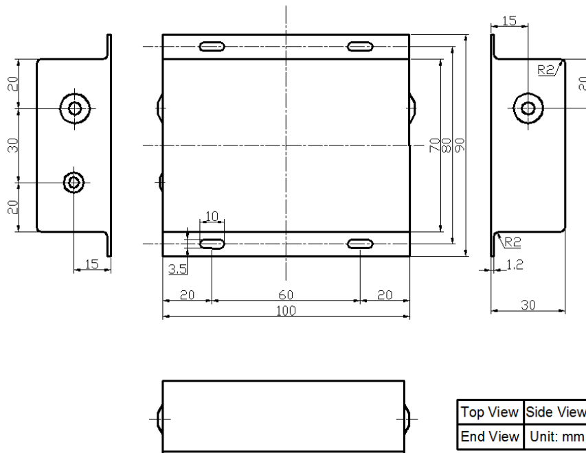
Figure 11. Dimensions for AHV24V10KV2MAW
