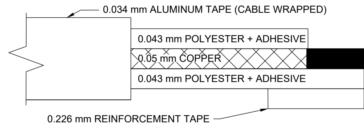
CROSS-SECTION
