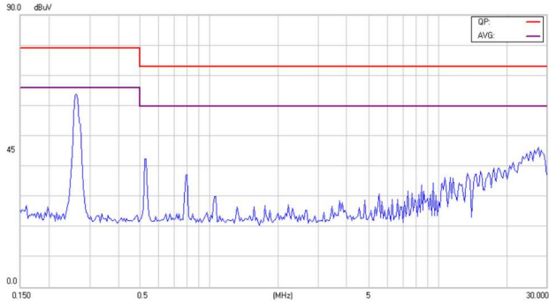
Conducted Class A of EC3SAW-48S05HP
