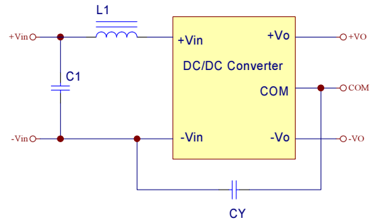
EC3SAWH dual output module
