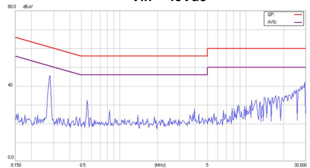
Conducted Class B of EC3SAW-48S15HP
