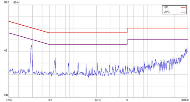
Conducted Class B of EC3SAW-24S33HP
