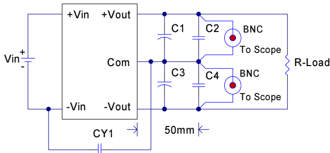
EC3SAWH Single Output Module
