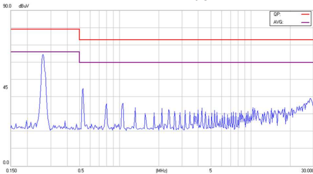
Conducted Class A of EC3SAW-24S05HP
