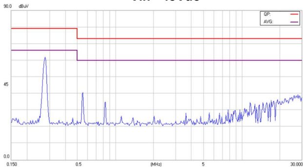
Conducted Class A of EC3SAW-48S15HP
