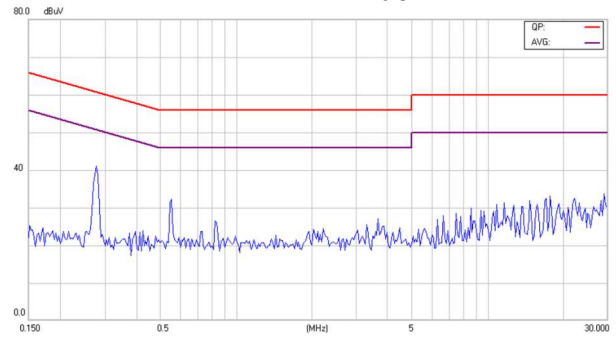
Conducted Class B of EC3SAW-24D15HP
