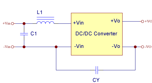
EC3SAWH single output module
