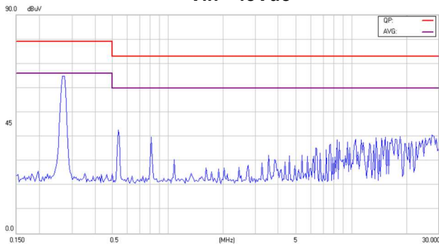
Conducted Class A of EC3SAW-48D15HP
