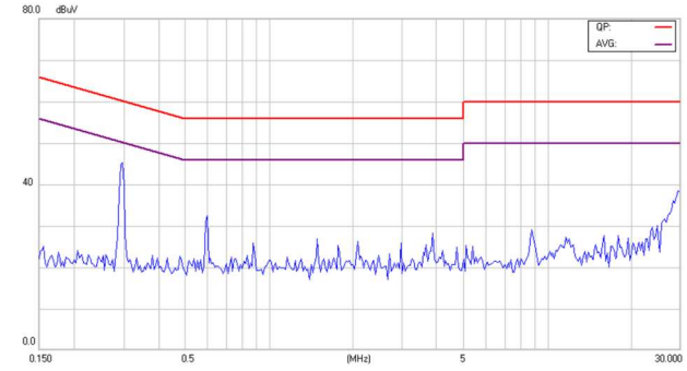
Conducted Class B of EC3SAW-24S12HP
