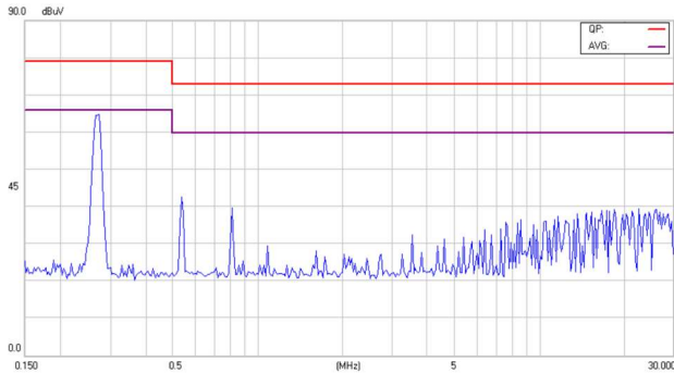
Conducted Class A of EC3SAW-48D12HP
