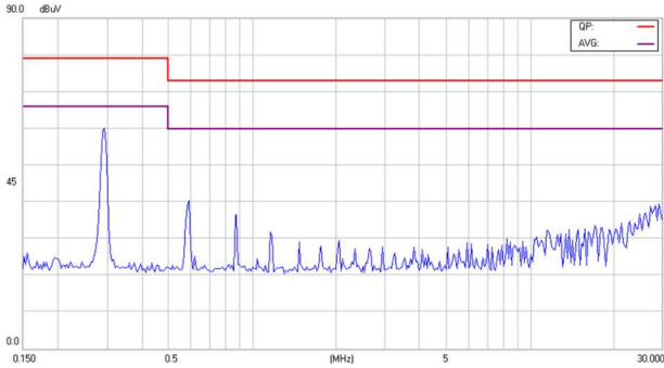
Conducted Class A of EC3SAW-24S33HP
