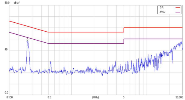
Conducted Class B of EC3SAW48S05HP
