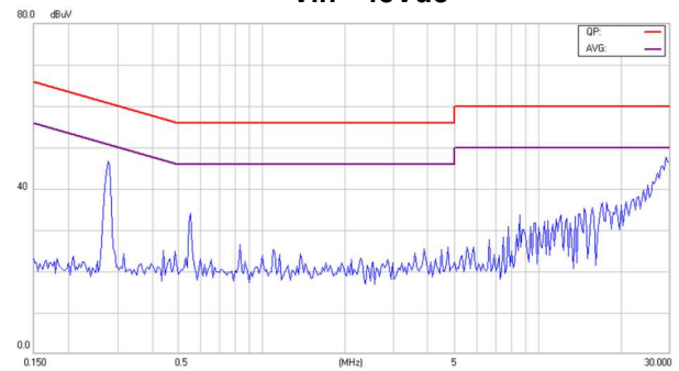
Conducted Class B of EC3SAW-48S12HP
