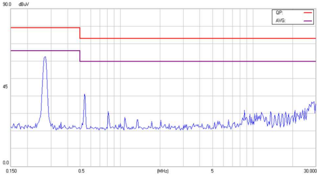
Conducted Class A of EC3SAW-24D05HP
