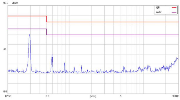
Conducted Class A of EC3SAW-24S12HP
