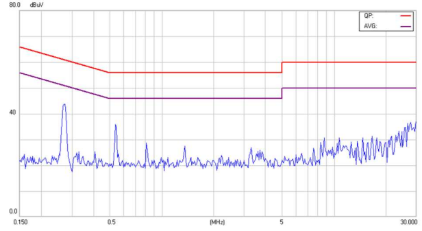
Conducted Class B of EC3SAW-24D05HP
