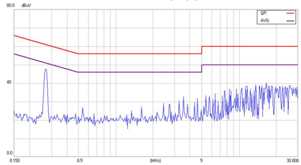
Conducted Class B of EC3SAW-48D12HP
