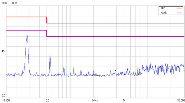
Conducted Class A of EC3SAW-24D15HP
