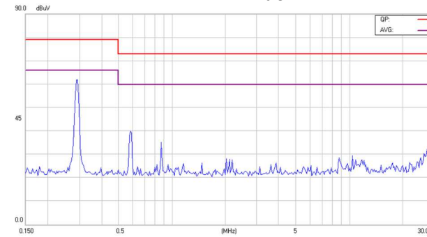
Conducted Class A of EC3SAW-24S15HP
