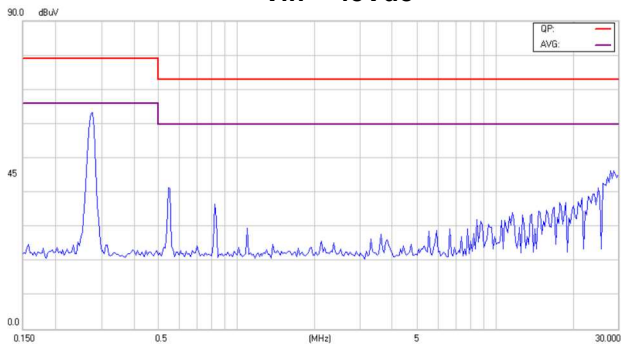
Conducted Class A of EC3SAW-48S12HP
