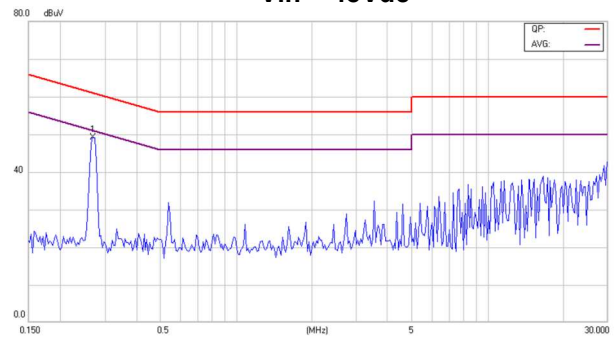
Conducted Class B of EC3SAW-48D15HP
