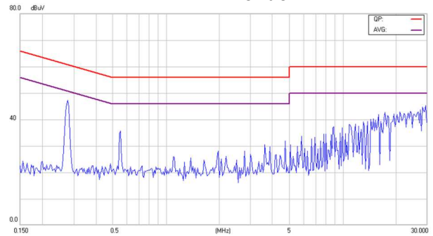
Conducted Class B of EC3SAW-48S33HP
