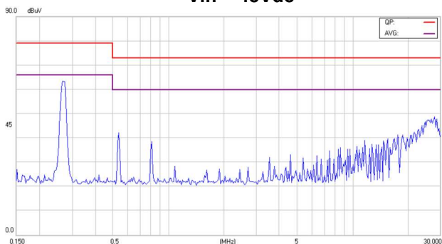
Conducted Class A of EC3SAW-48D05HP
