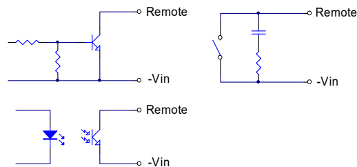
Remote On/Off Connection Examples
