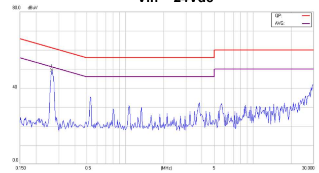
Conducted Class B of EC3SAW-24S05HP
