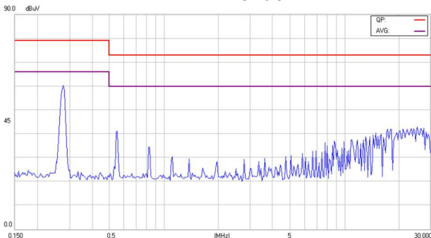
Conducted Class A of EC3SAW-48S33HP
