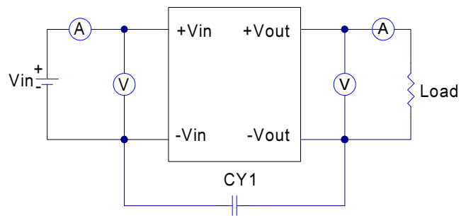
EC3SAWH Series Test Setup
