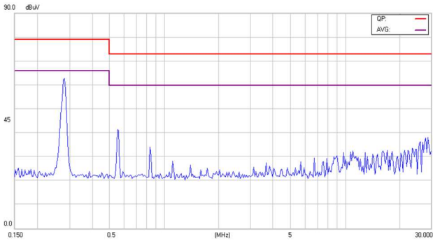
Conducted Class A of EC3SAW-24D12HP
