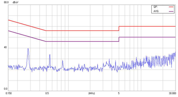
Conducted Class B of EC3SAW-24D12HP
