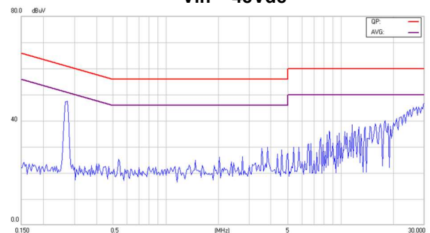
Conducted Class B of EC3SAW48D05HP
