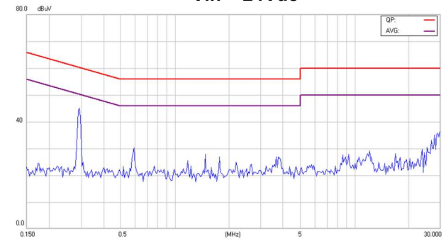
Conducted Class B of EC3SAW-24S15HP
