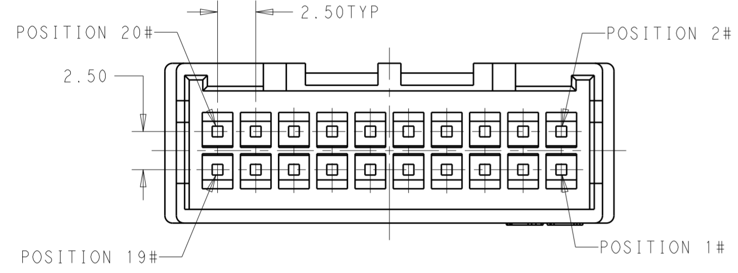
DUAL LATCH DETAIL FOR 1-2324201-8 THROUGH 4-2324201-0
