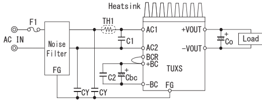
Fig.1.1 Connection for standard use
