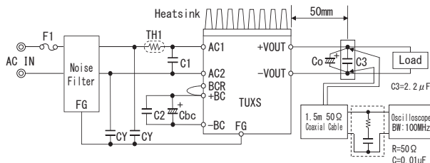
Fig.2.1 Method of Measuring Output Ripple and Ripple Noise
