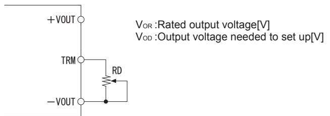
Fig. 3.2 Connection for output voltage decreasing
