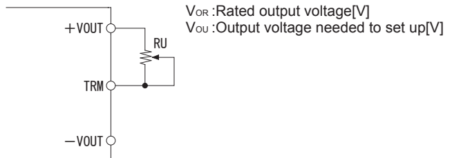
Fig. 3.3 Connection for output voltage increasing
