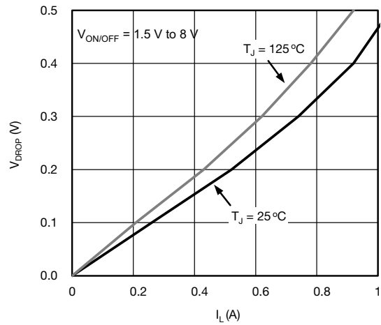
V_{DROPP} vs. I_L at V_{IN} = 1.8\text{ V}
