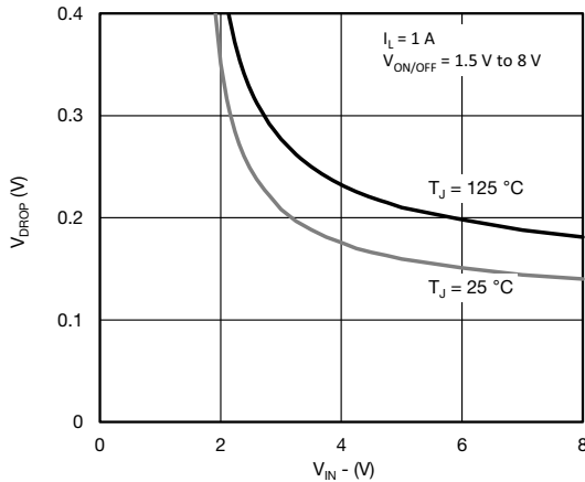
V_{DROPP} vs. V_{IN} at I_L = 1\text{ A}
