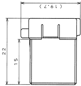
SECT. A-A
