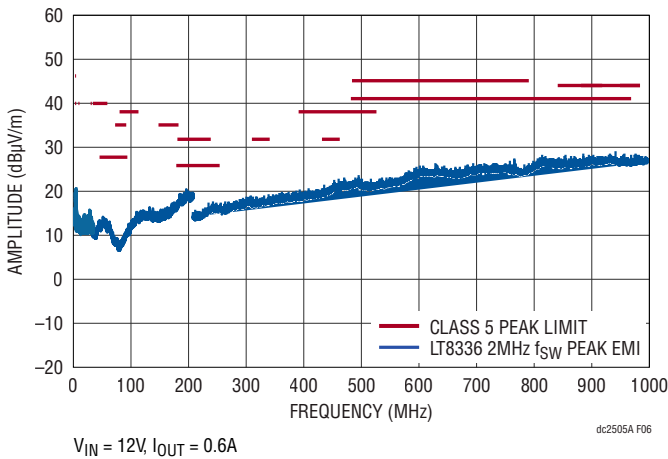
Figure 6. Radiated Emission Test (CISPR25 Class 5 Peak)
