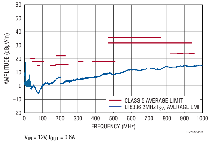
Figure 7. Radiated Emission Test (CISPR25 Class 5 Peak Average)
