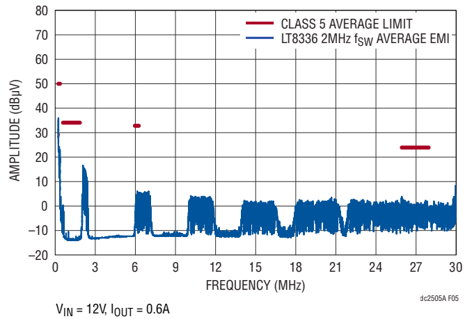
Figure 5. Conducted Emission Test (CISPR25 Class 5 Peak Average)
