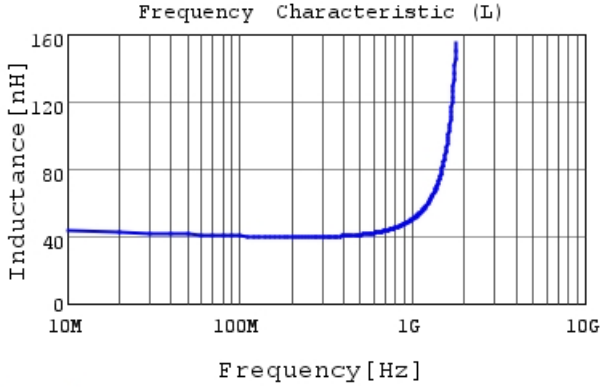
LQG15WZ40NG02 L
