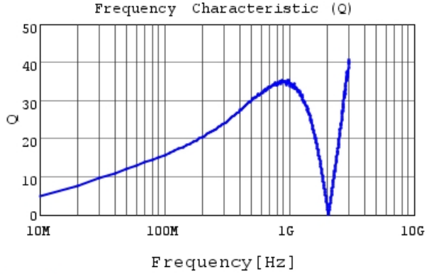
LQG15WZ40NG02 Q
