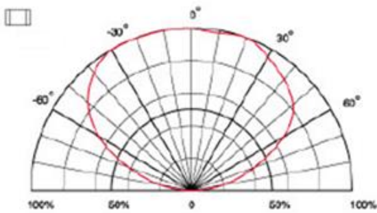
Directive Characteristics
