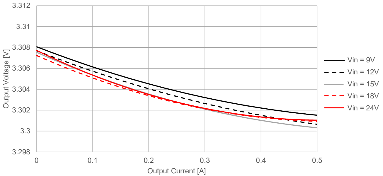
173950336 Load Regulation V_{OUT} = 3.3V , T_A = 25^\circ C
