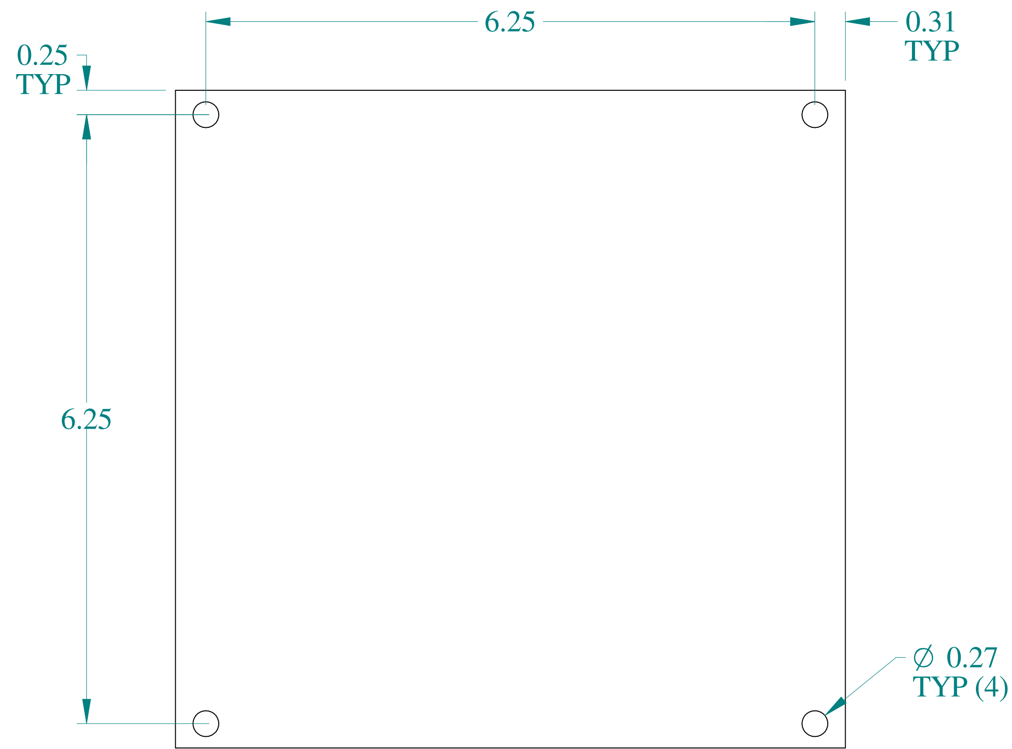
FRONT VIEW
