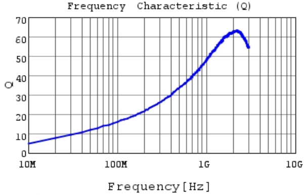
LQG15WZ5N8C02 Q
