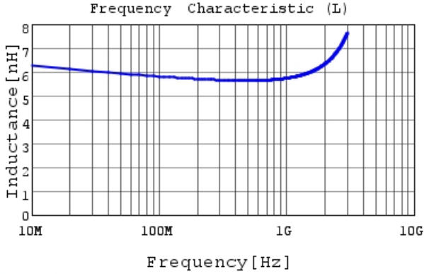
LQG15WZ5N8C02 L
