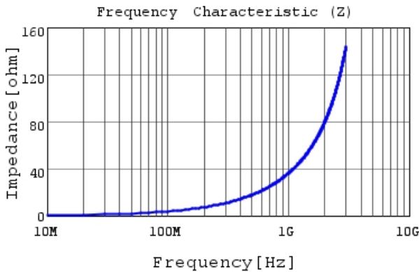
LQG15WZ5N8C02 |Z|
