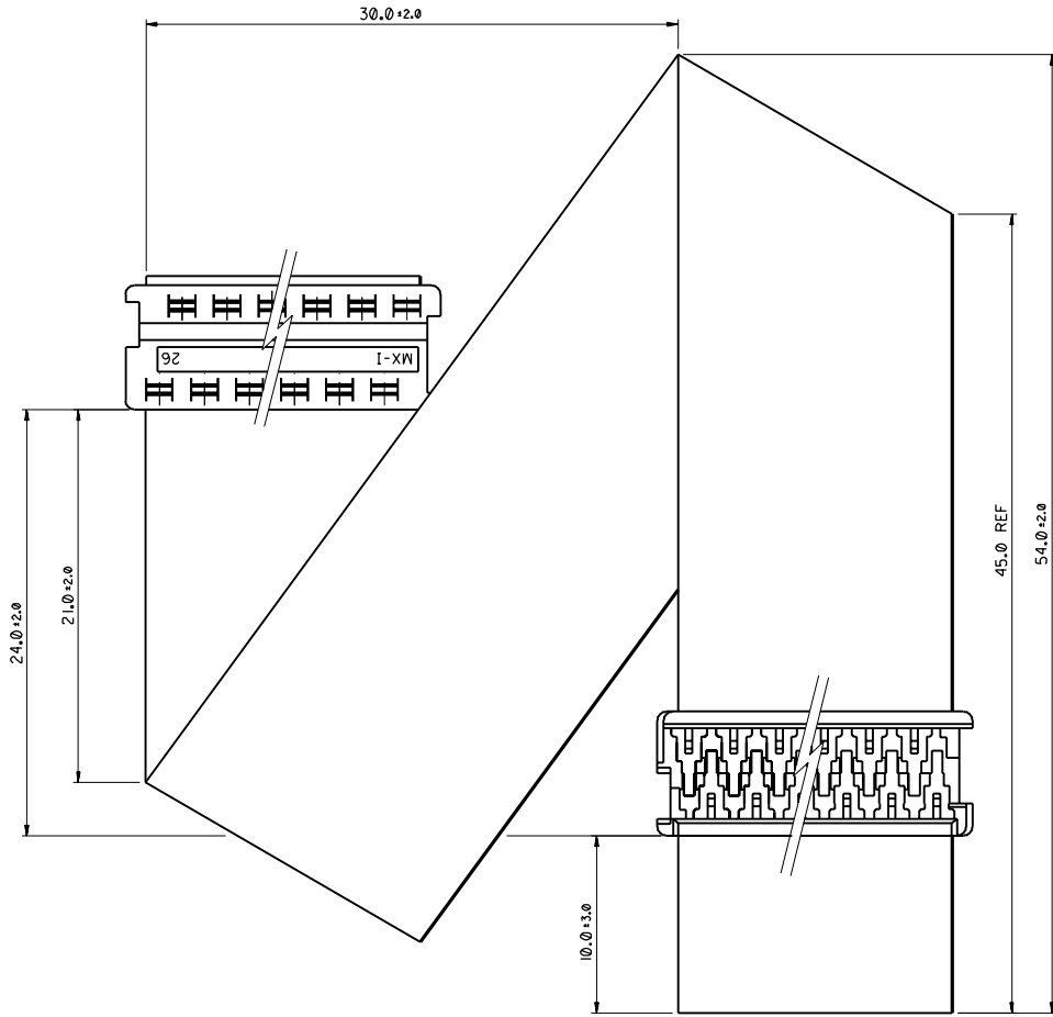
FOLDED CABLE HARNESS
