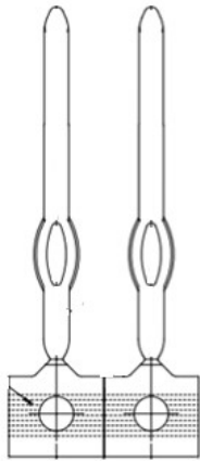
43886 compliant pin
