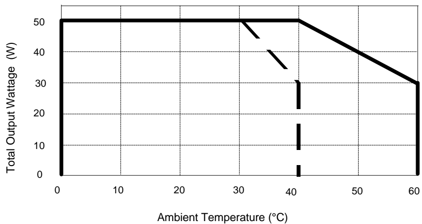
OUTPUT DERATING CURVE Convection Cooling
