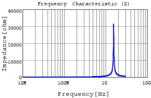
LQG15WZ72NJ02 |Z|
