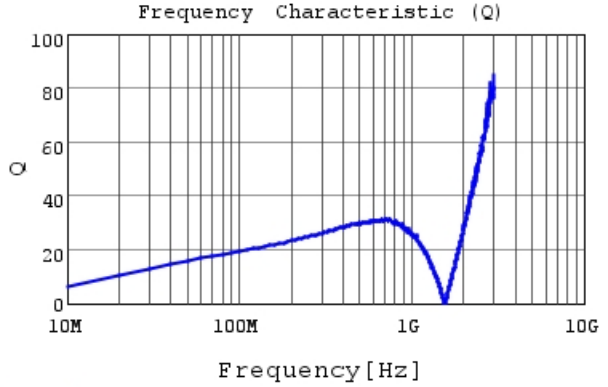
LQG15WZ72NJ02 Q
