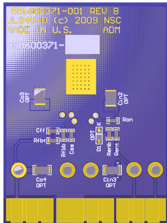
Figure 4-2. Back View
