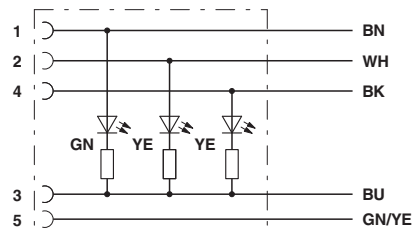
Contact assignment of M12 socket, with exception of conductor types 115, 186, 515, 520, and 800. Here, the fifth wire is gray and not green/yellow.
