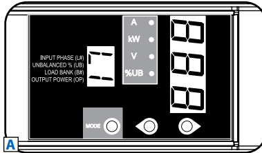
Multifunction Load Meter: Displays the load for each phase, bank or total output; rotate the display 180°.
