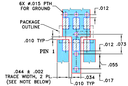
Demo Board MCL P/N: TB-285 Suggested PCB Layout (PL-158)
