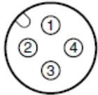
M12 Connector Pin Arrangement
