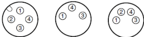
M12 Connector Pin Arrangement (See note 2.) M8 connector (3 pin) Pin Arrangement M8 Connector (4 pin) Pin Arrangement (See note 2.)
