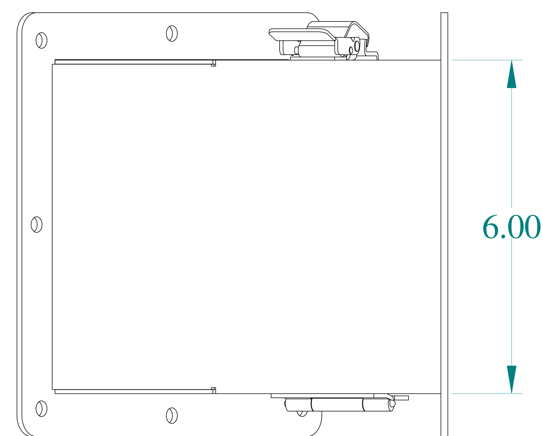
BOTTOM VIEW
