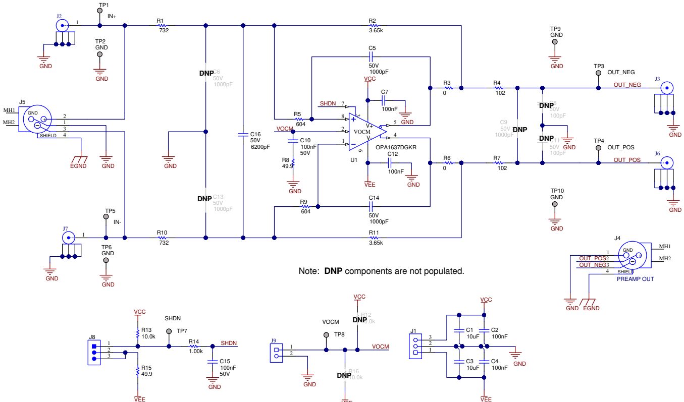
Figure 1. OPA1637EVM Schematic
