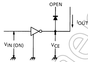
5. V_{IN} (ON)
