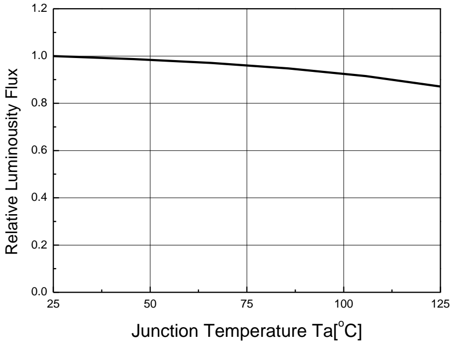
Fig 6. Relative Light Output vs. Junction Temperature, I_F=100\text{mA}
