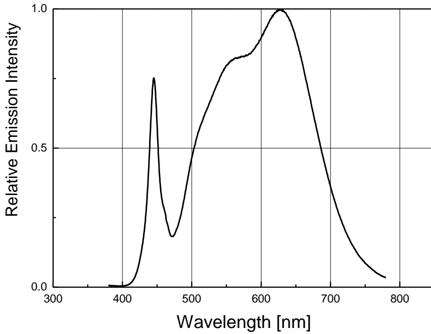
Fig 1. Color Spectrum, I_F=100\text{mA} , T_j = 25^\circ\text{C} , RH30%
