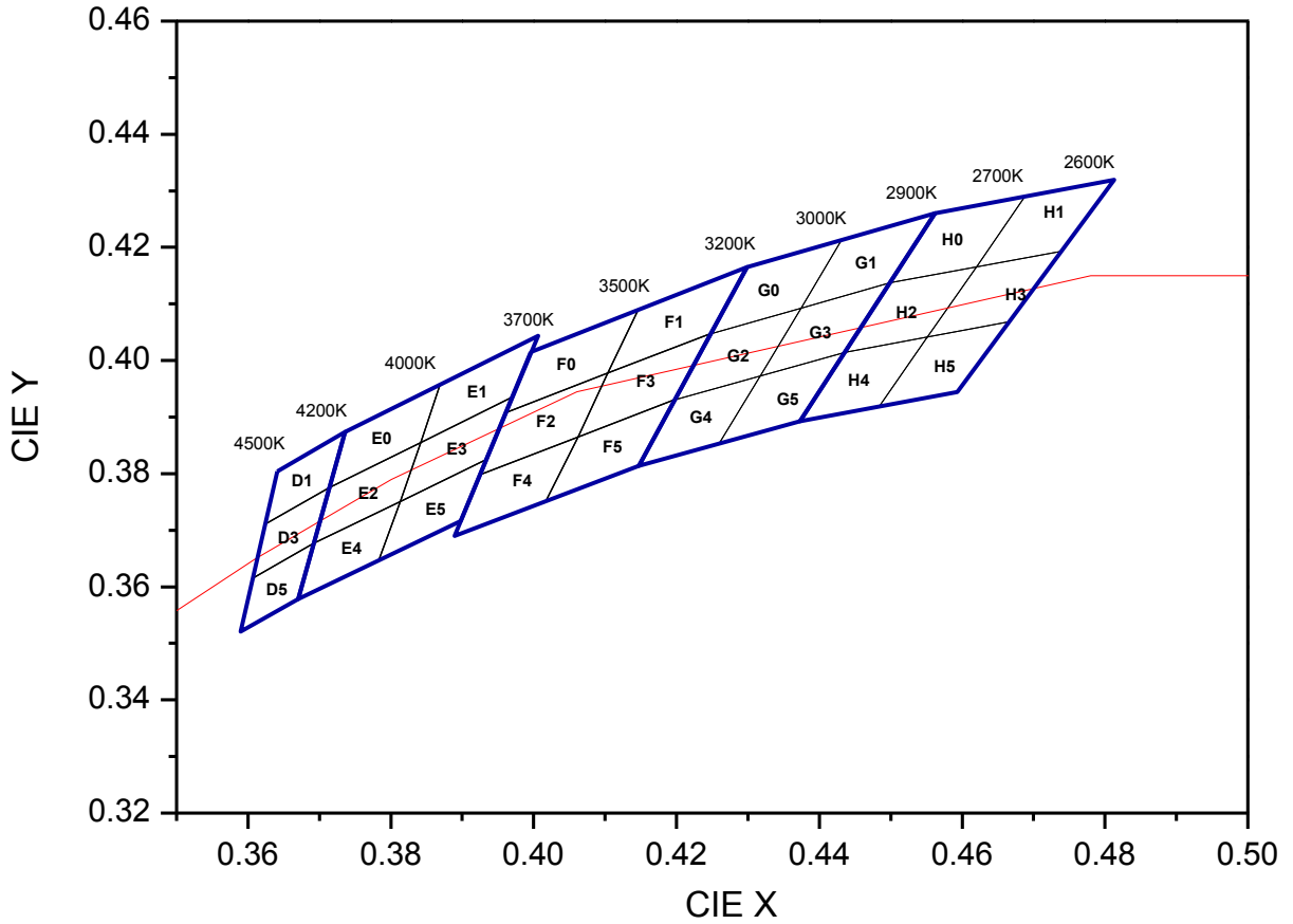
CIE Chromaticity Diagram, I_F = 100\text{mA} , T_j = 25^\circ\text{C}
