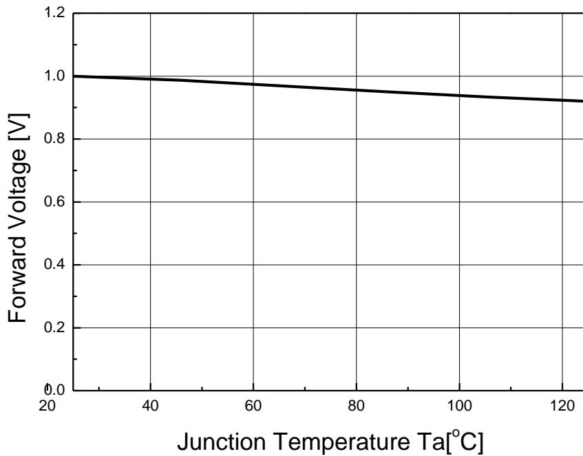
Fig 7. Junction Temperature vs. Relative Forward Voltage, I_F=100\text{mA}
