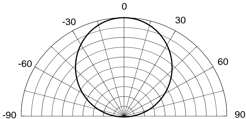
Fig 2. Viewing Angle Distribution, T_a=25^\circ\text{C}
