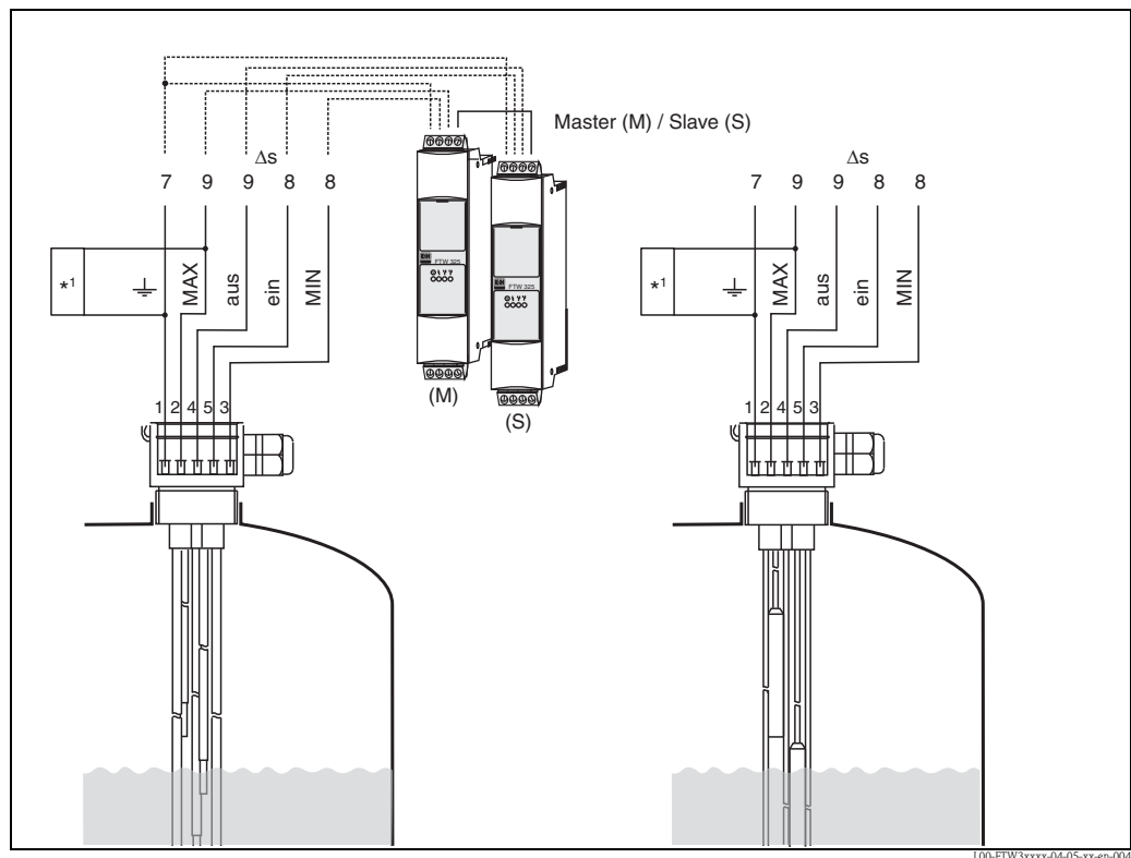
*1 Printed circuit board for cable monitoring (only required for probes with WHG certification.) The power supply and evaluation are provided by a switching unit, e.g. Nivotester FTW325
