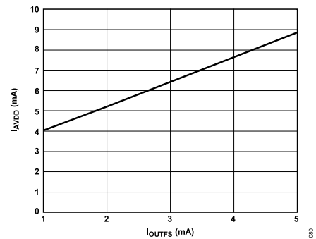
Figure 80. I AVDD vs. I OUTFS at AVDD = 3.3 V
