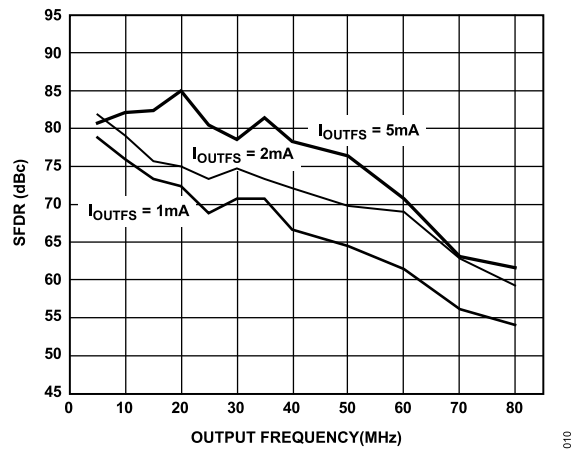
Figure 12. SFDR vs. f_{OUT} and I_{OUTFS} at 175 MSPS
