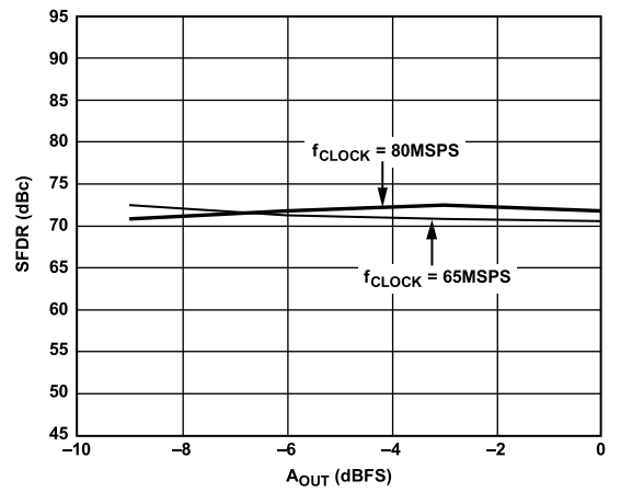
Figure 32. SFDR vs. A_{OUT} at f_{OUT} = f_{CLOCK}/5
