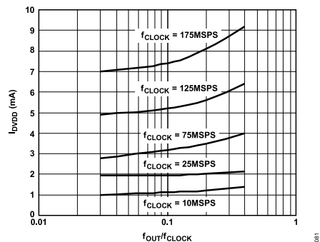
Figure 82. I DVDD vs. f OUT /f CLOCK Ratio at DVDD = 3.3 V
