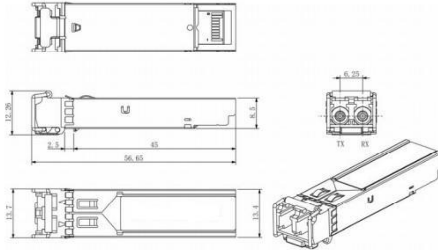
Mechanical Drawing
