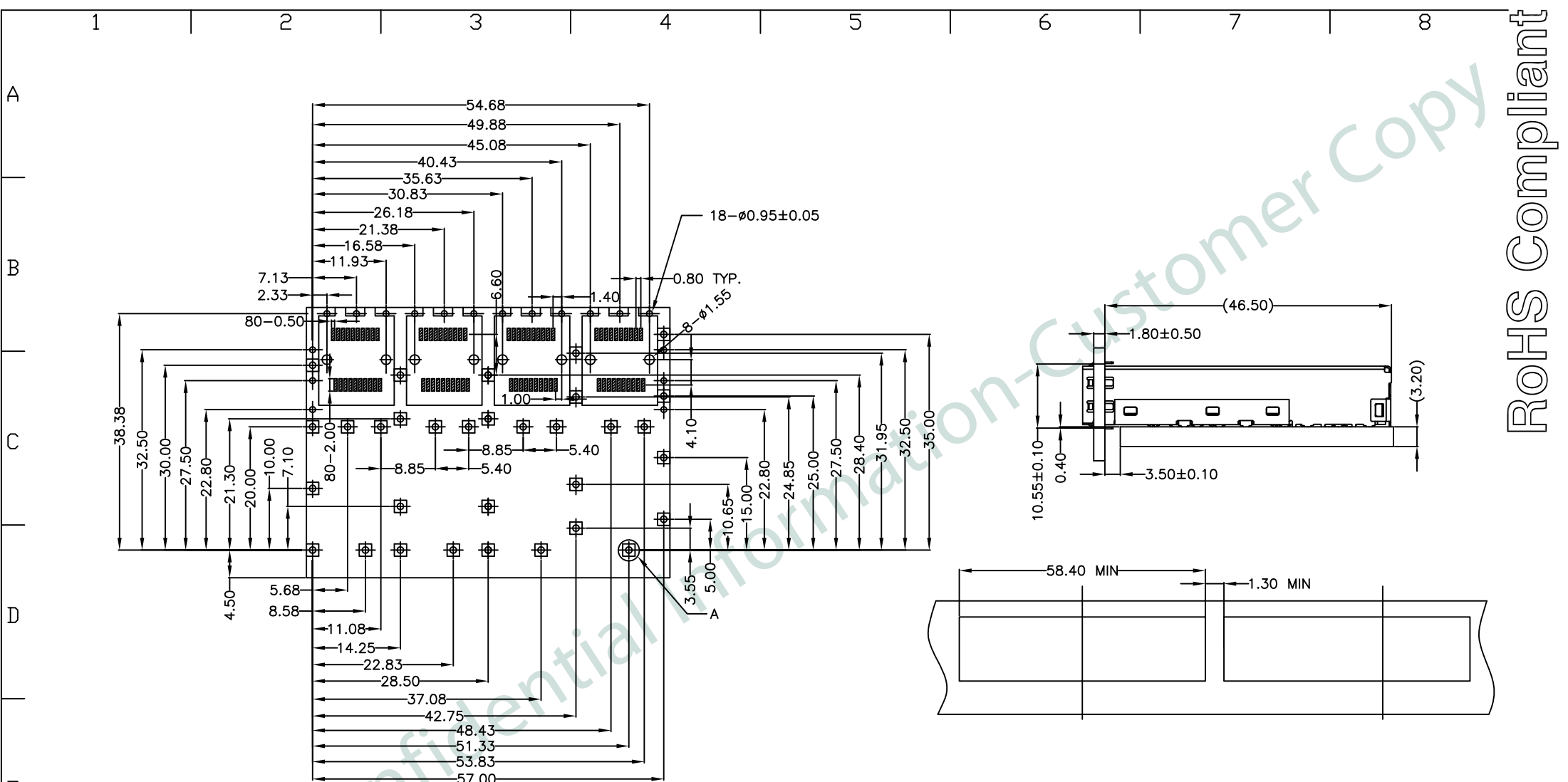
P.C.B LAYOUT TOP VIEW ±0.05
