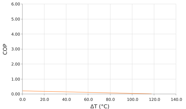
Coefficient of Performance (COP = Qc/Pin) Thot = 27 °C | Current = 1.5 Amps
