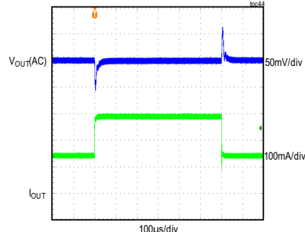
MAXM17906 LOAD TRANSIENT RESPONSE V_{IN} = 12V , ADJUSTABLE V_{OUT} = 1.5V , PWM MODE (LOAD CURRENT STEPPED FROM 150mA TO 300mA)
