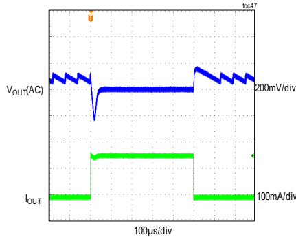
MAXM17906 LOAD TRANSIENT RESPONSE V_{IN} = 12V , ADJUSTABLE V_{OUT} = 5V , PFM MODE (LOAD CURRENT STEPPED FROM 5mA TO 150mA)
