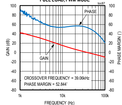
MAXM17906 BODE PLOT
