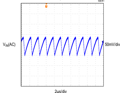
MAXM17904 INPUT VOLTAGE RIPPLE V_{IN} = 12V , FIXED V_{OUT} = 3.3V , FULL LOAD, PWM MODE
