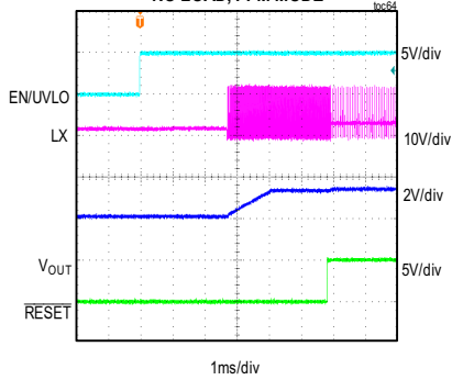
MAXM17904 STARTUP THROUGH ENABLE: 2V PREBIAS V_{IN} = 12V , FIXED V_{OUT} = 3.3V , NO LOAD, PFM MODE
