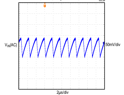
MAXM17906 INPUT VOLTAGE RIPPLE V_{IN} = 12V , ADJUSTABLE V_{OUT} = 3.3V , FULL LOAD, PWM MODE
