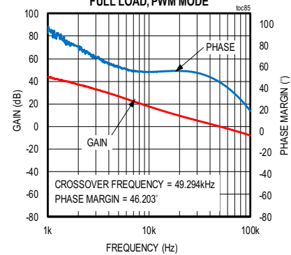
MAXM17906 BODE PLOT
