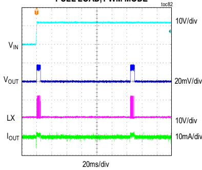
MAXM17904 OUTPUT SHORT DURING STARTUP V_{IN} = 12V , FIXED V_{OUT} = 3.3V , FULL LOAD, PWM MODE
