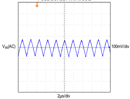
MAXM17906 INPUT VOLTAGE RIPPLE V_{IN} = 12V , ADJUSTABLE V_{OUT} = 5V , FULL LOAD, PWM MODE
