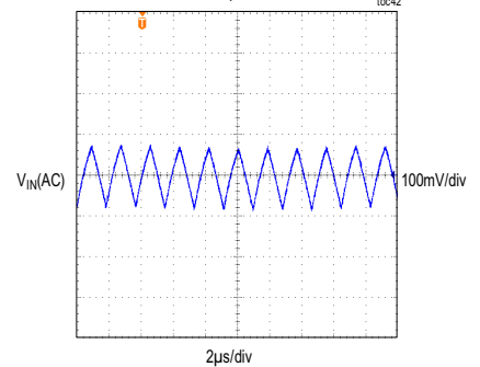
MAXM17905 INPUT VOLTAGE RIPPLE V_{IN} = 12V , FIXED V_{OUT} = 5V FULL LOAD, PWM MODE
