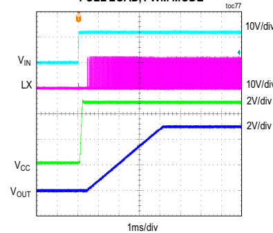
MAXM17905 STARTUP THROUGH V_{IN} V_{IN} = 12V , FIXED V_{OUT} = 5V , FULL LOAD, PWM MODE
