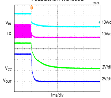
MAXM17906 SHUTDOWN THROUGH V_{IN} V_{IN} = 12V , ADJUSTABLE V_{OUT} = 5V , FULL LOAD, PWM MODE
