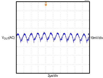
MAXM17905 OUTPUT VOLTAGE RIPPLE V_{IN} = 12V , FIXED V_{OUT} = 5V FULL LOAD, PWM MODE
