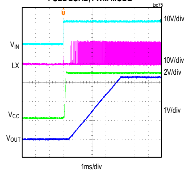
MAXM17904 STARTUP THROUGH V_{IN} V_{IN} = 12V , FIXED V_{OUT} = 3.3V , FULL LOAD, PWM MODE
