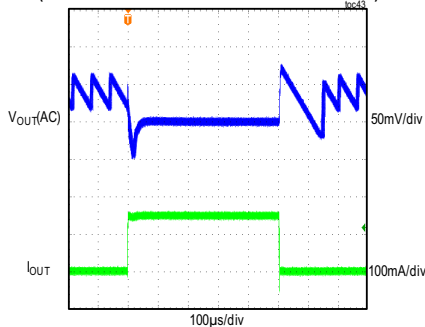
MAXM17906 LOAD TRANSIENT RESPONSE V_{IN} = 12V , ADJUSTABLE V_{OUT} = 1.5V , PFM MODE (LOAD CURRENT STEPPED FROM 5mA TO 150mA)
