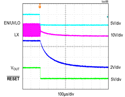
MAXM17905 SHUTDOWN THROUGH ENABLE V_{IN} = 12V , FIXED V_{OUT} = 5V , FULL LOAD, PWM MODE
