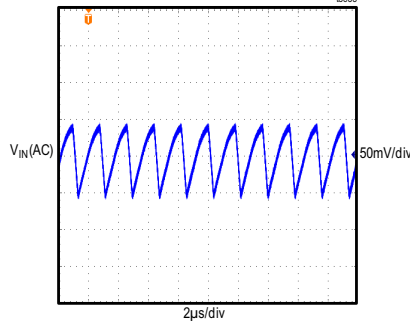
MAXM17906 INPUT VOLTAGE RIPPLE V_{IN} = 12V , ADJUSTABLE V_{OUT} = 1.5V FULL LOAD, PWM MODE
