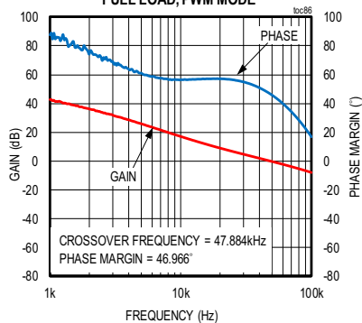
MAXM17906 BODE PLOT V_{IN} = 12V , ADJUSTABLE V_{OUT} = 3.3V , FULL LOAD, PWM MODE
