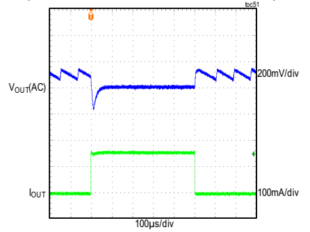
MAXM17905 LOAD TRANSIENT RESPONSE V_{IN} = 12V , FIXED V_{OUT} = 5V , PFM MODE (LOAD CURRENT STEPPED FROM 5mA TO 150mA)
