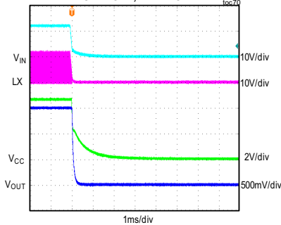
MAXM17906 SHUTDOWN THROUGH V_{IN} V_{IN} = 12V , ADJUSTABLE V_{OUT} = 1.5V , FULL LOAD, PWM MODE
