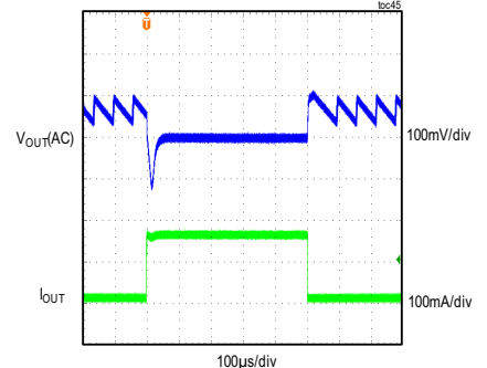
MAXM17906 LOAD TRANSIENT RESPONSE V_{IN} = 12V , ADJUSTABLE V_{OUT} = 3.3V , PFM MODE (LOAD CURRENT STEPPED FROM 5mA TO 150mA)
