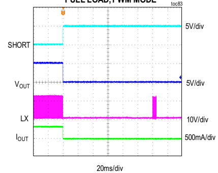
MAXM17905 OUTPUT SHORT IN STEADY STATE V_{IN} = 12V , FIXED V_{OUT} = 5V , FULL LOAD, PWM MODE
