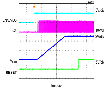
MAXM17905 STARTUP THROUGH ENABLE V_{IN} = 12V , FIXED V_{OUT} = 5V , FULL LOAD, PWM MODE
