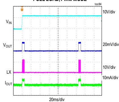
MAXM17905 OUTPUT SHORT DURING STARTUP V_{IN} = 12V , FIXED V_{OUT} = 5V , FULL LOAD, PWM MODE
