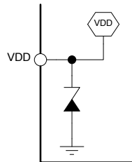
TYPE 8: VDD Power Supply
