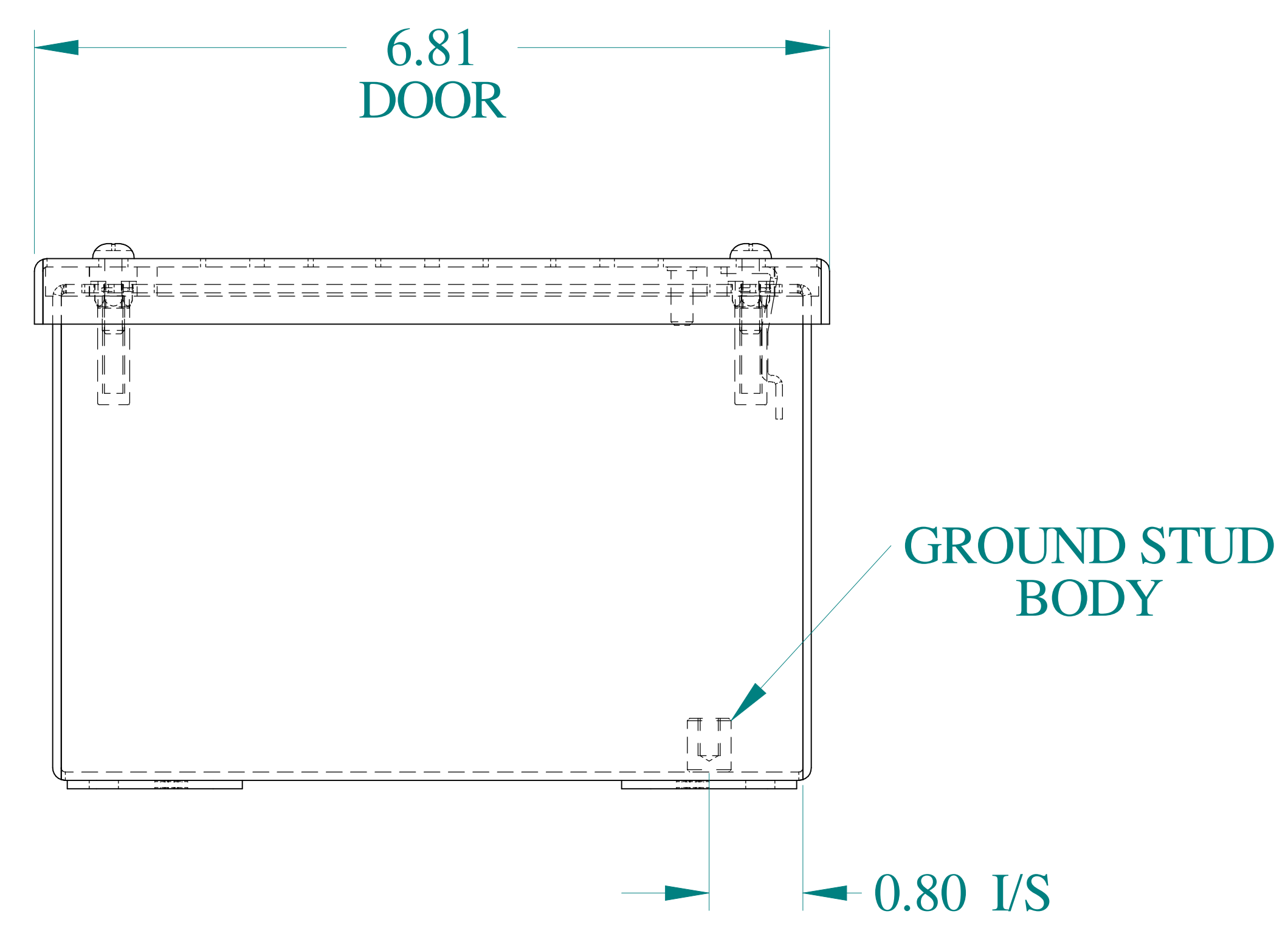
BOTTOM VIEW
