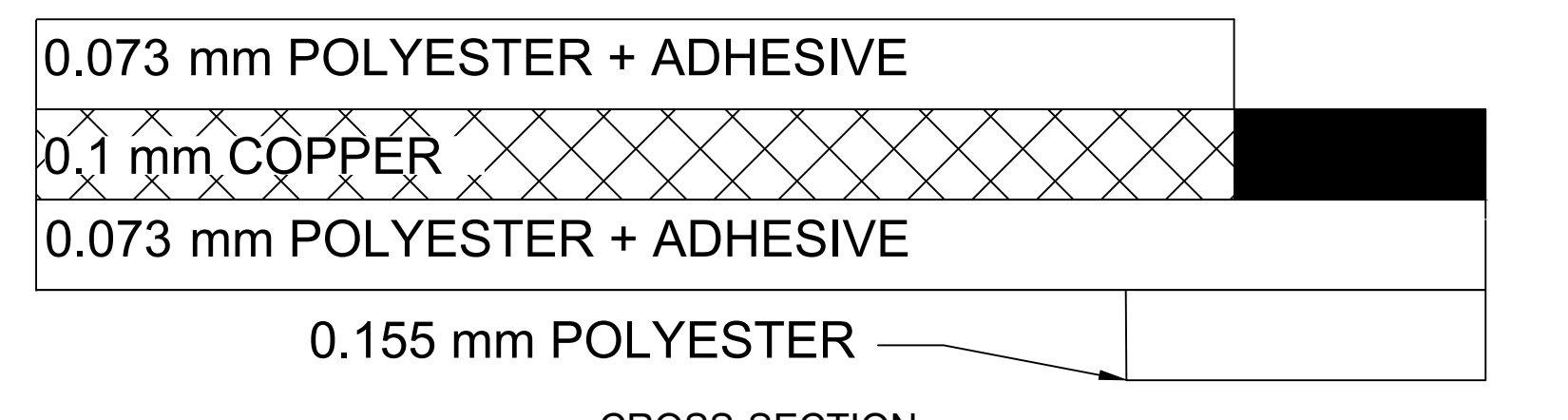
CROSS-SECTION
