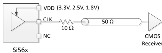
Single CMOS Termination
