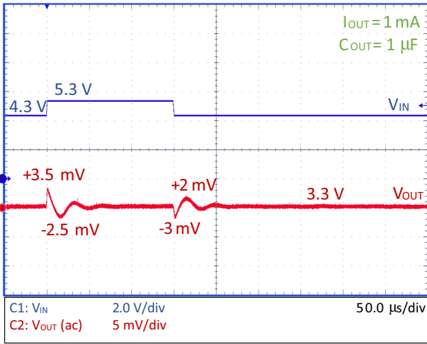
Figure 32. Line Transient – NCP730–3.3 V
