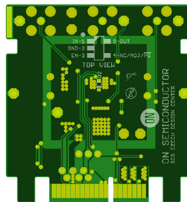
Figure 92. TSOP-5 Demo Board (2 layer, rev. 1) – PCB Bottom Layer
