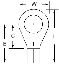
MU10-516R/S Stud Size 5/16 Wire Range 12-10
