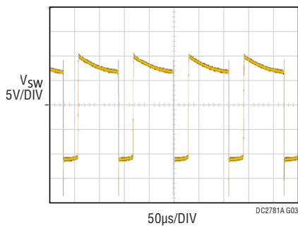
Figure 5. Steady State Switch Node Voltage at 19V Full Load Condition
