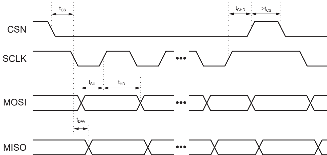
Figure 4: SPI Timing
