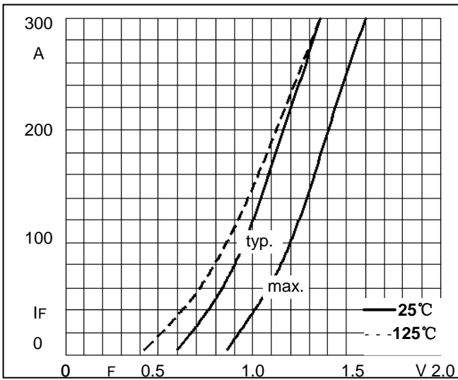
Fig1. Forward Characteristics
