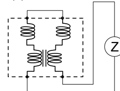
(C) Differential mode
